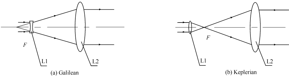
Fig. 1 Expand system of Galilean telescope and Keplerian telescope
