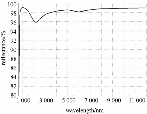
Fig. 6 Theoretical index of reflection for golden enhanced mirror
